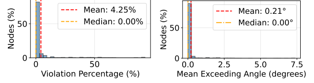
Figure 6. CLIP image embeddings for ImageNet are tightly clustered. (Left): For a fixed node i , we show the proportion of non-descendants of i whose embeddings intersect the cone of i . (Right): For the same node i , we show the mean angle violation, with non-violating angles counted as 0.
